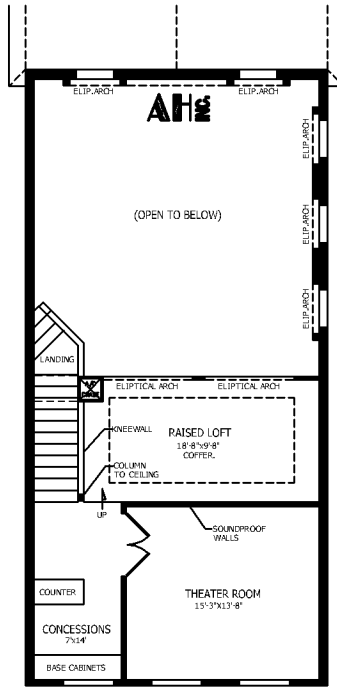
2ND FLOOR OPTION "B"
